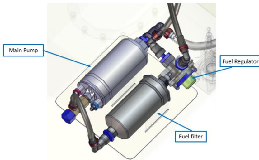
Main pump & fuel filter scheme (SPEC.2):
