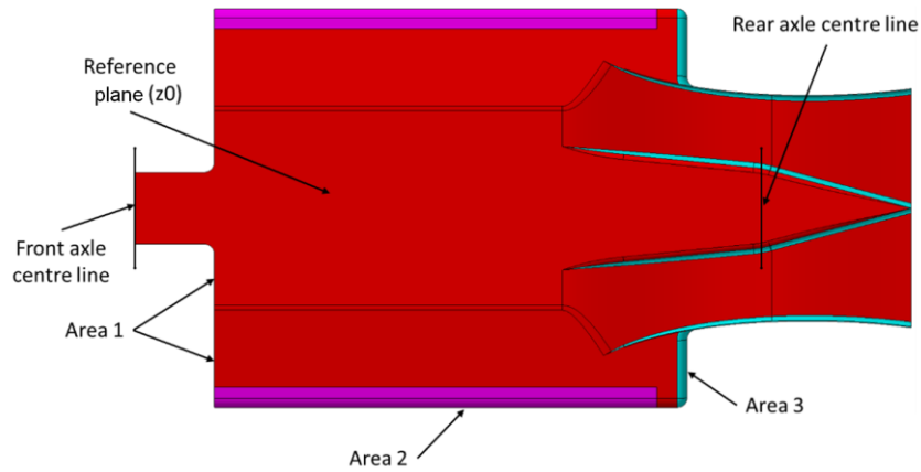
Base underfloor with diffuser add-ons and free boxes:
