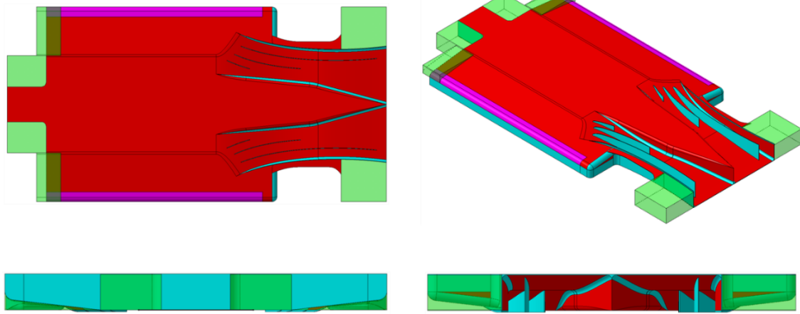
Base underfloor with diffuser add-ons and free boxes:
